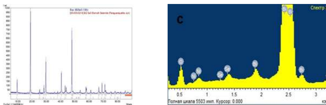
Fig. 1. X-ray diffraction pattern (a) and elemental composition (b) of \text{Bi}_2\text{Se}_3 thin films obtained from ethylene glycol. Electrolyte composition (M): 0.07 \text{ Bi}(\text{NO}_3)_3 \cdot 5\text{H}_2\text{O} + 0.03 \text{ H}_2\text{SeO}_3 + \text{C}_6\text{H}_8\text{O}_7 ; T=298\text{K} . E_V=0.02 \text{ V/s} .
