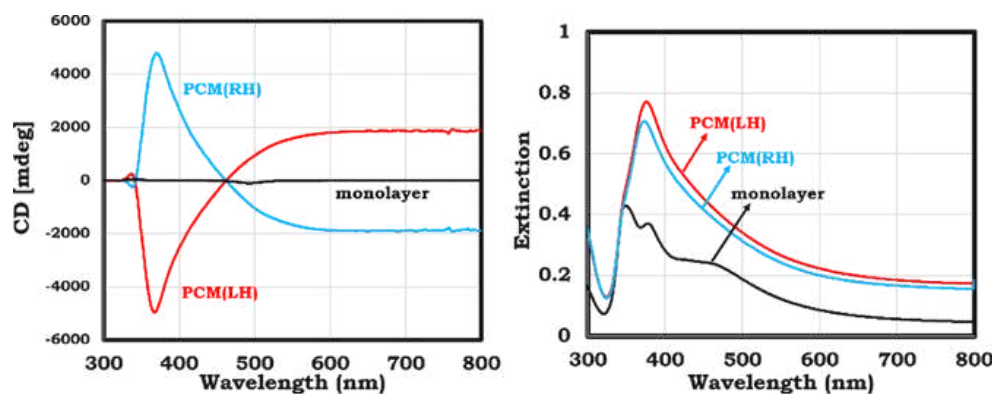
Figure 1. Grazing Incidence Spraying, Layer by Layer Assembly, Integrated flow cell, Circular dichroism and extinction spectra of plasmonic chiral metasurface (PCM)
