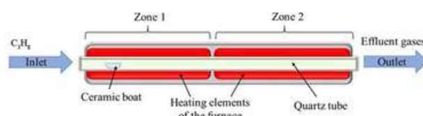
Fig. 1. Schematic representation of cross-section of the furnace during the synthesis of carbon nanotubes with propane feedstock.
