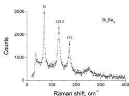
Fig. 2. Raman spectrum for \text{Bi}_2\text{Se}_3 samples
