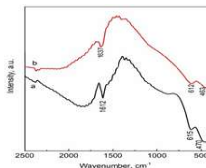
Fig. 3. FTIR spectra of \text{Bi}_2\text{Se}_3 : a) powder; b) thin film
